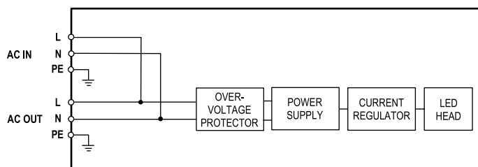
LI-10-230-F block diagram
